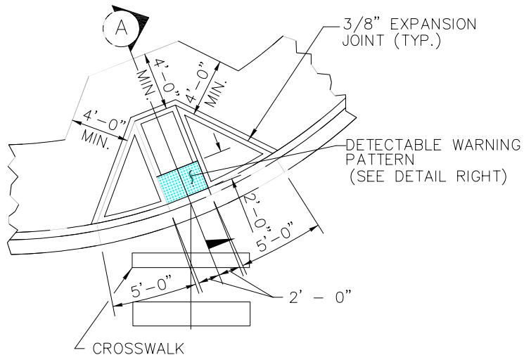
CURB RAMP TYPE 3 PLAN
