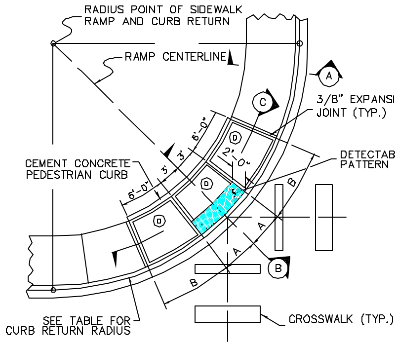
CURB RAMP TYPE 2 PLAN
