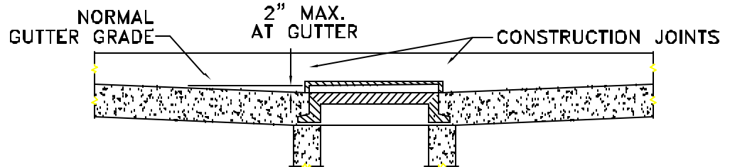
SECTION B-B
