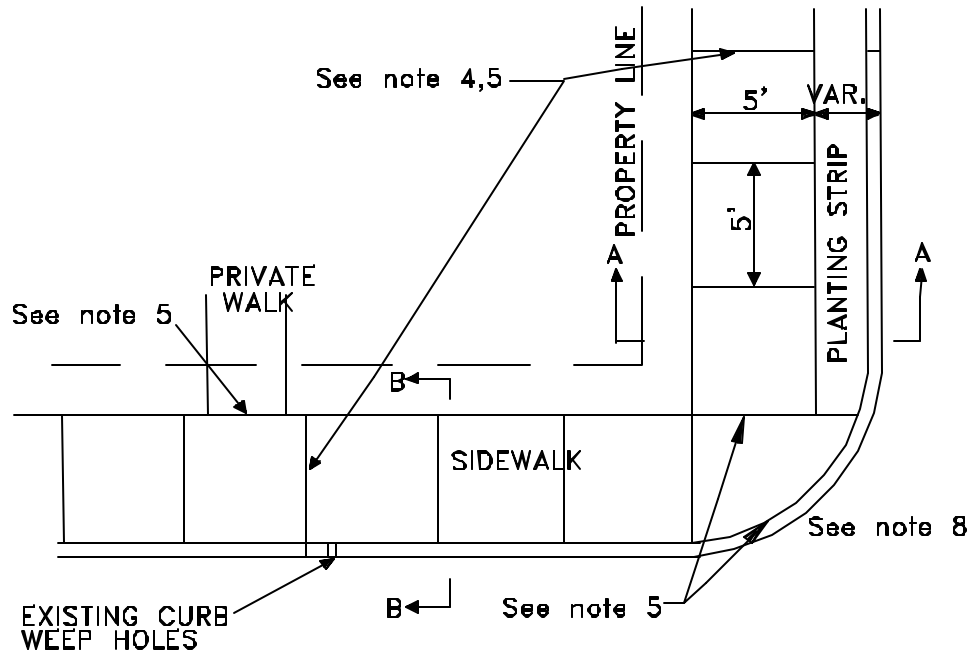
PLAN VIEW
