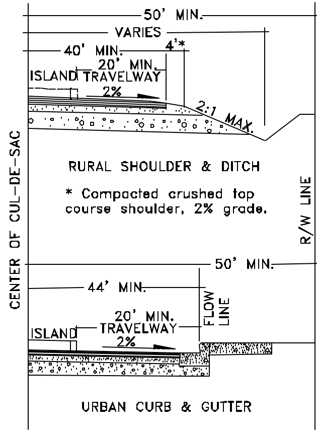
DRAWING 505.L-1 CUL-DE-SAC & INTERSECTION DETAIL WHATCOM COUNTY DEPARTMENT OF PUBLIC WORKS
